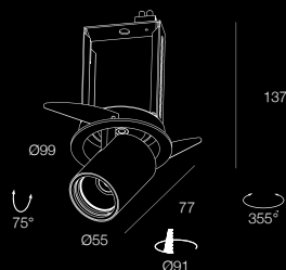
9.1W 350mA 1388lm, CRI80 COB LED
